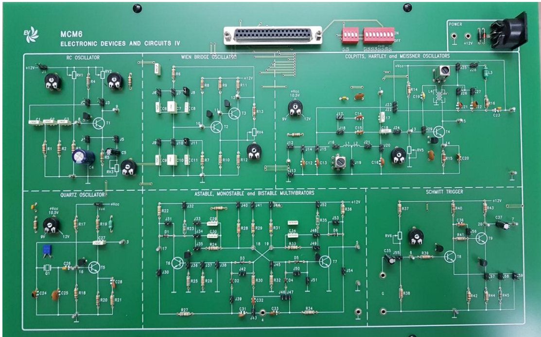
Oscillator Circuit Module
