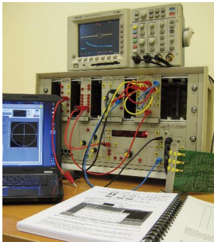
Wireless Communication and Signal Trainer
