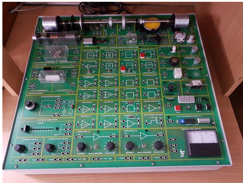
Transducer Module
