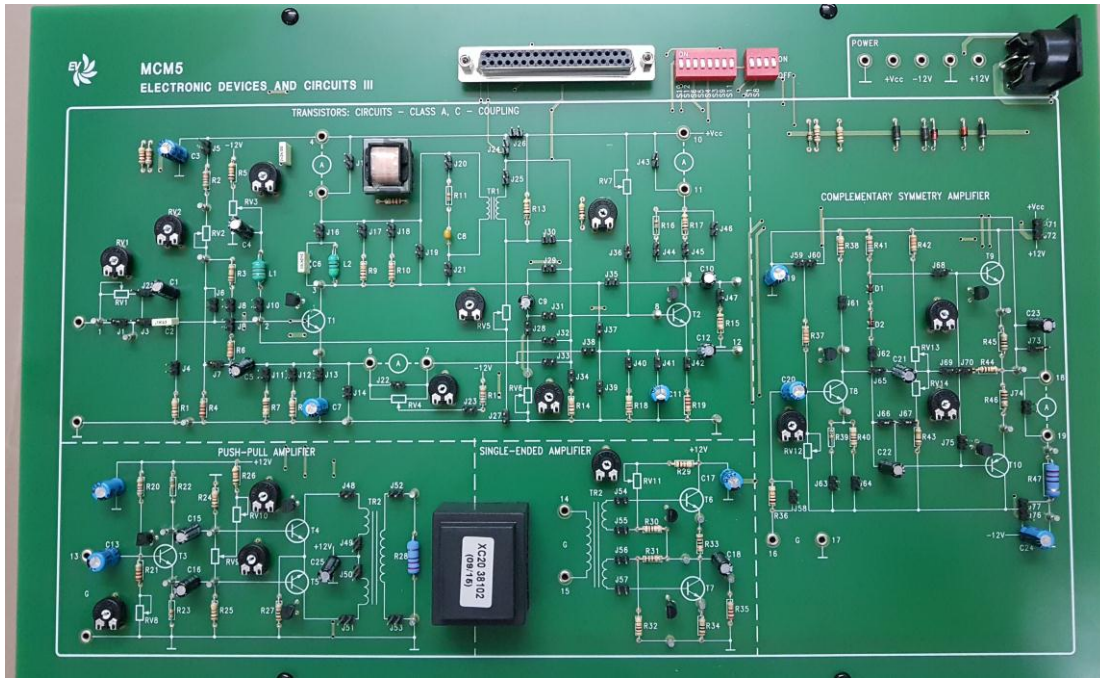
Power Amplifier Module
