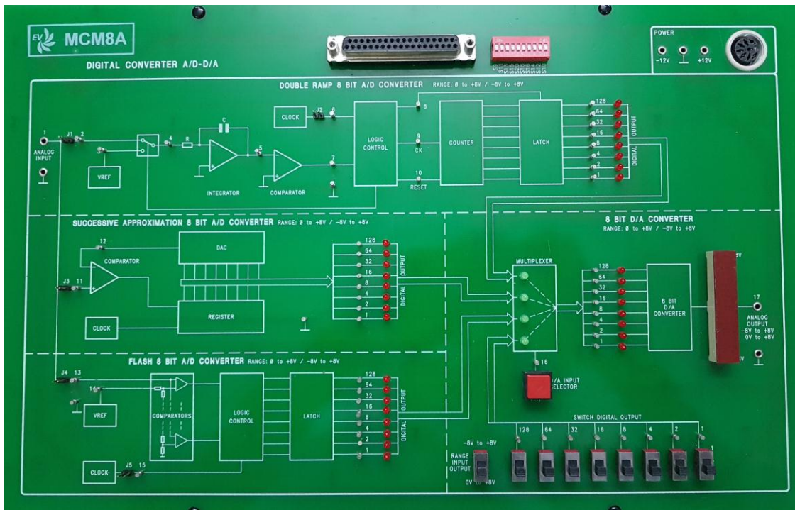
Digital to Analog and Analog to Digital Converter
