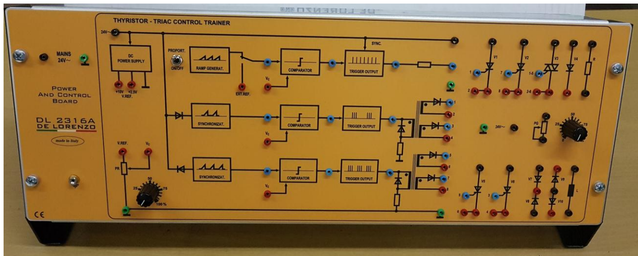
Power and Control Board Module
