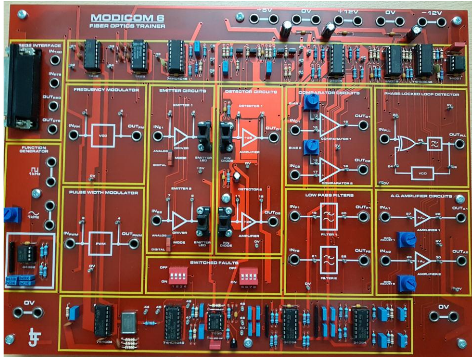
Optical Fiber Trainer Module
