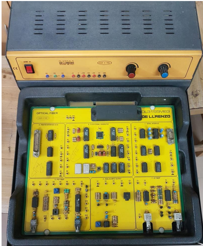
PC based Mobile Telephony Trainer
