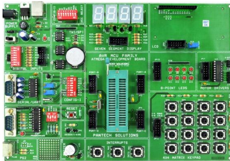
Micro controller Development Board
